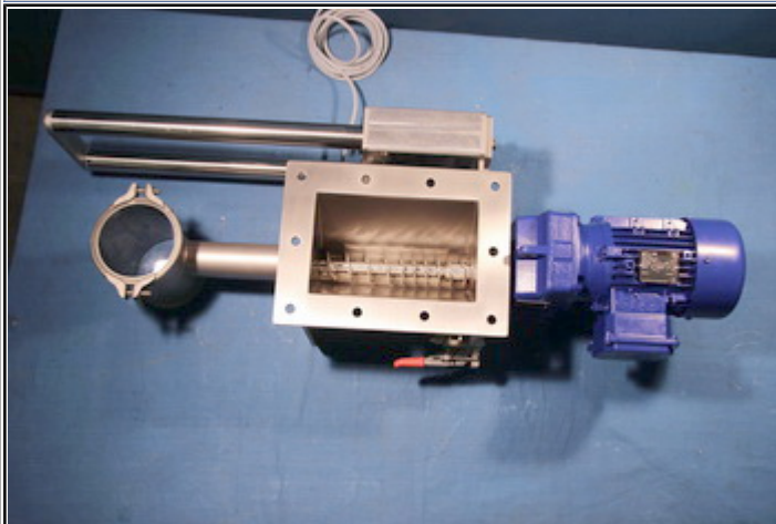
Screw feeder with thread extraction device
